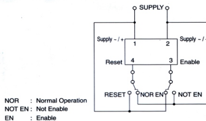
DIGITAL HOUR METER
