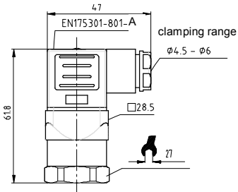
connector according to DIN EN 175301 – 803 Form A
