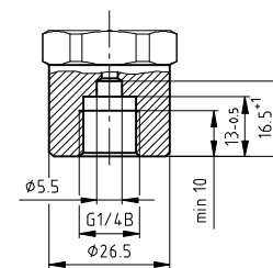
G 1/4 female
