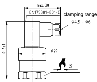
connector according to DIN EN 175301 – 803 Form C
