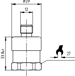
circular plug-in connector M12x1
